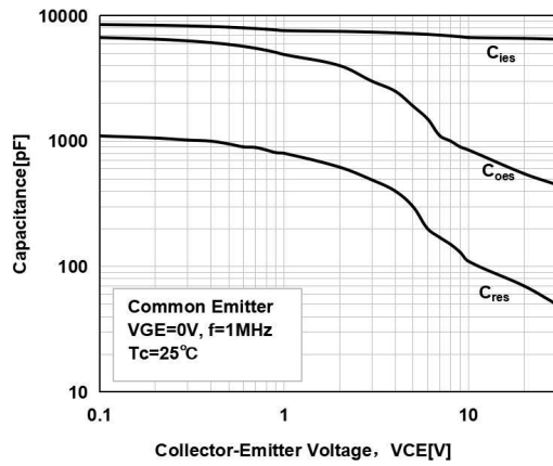
Capacitance Characteristics
